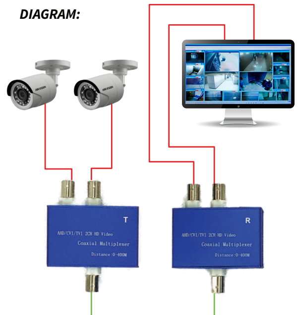
Single core coaxial cable SYV75-5-10-400M adaptive adjustment
