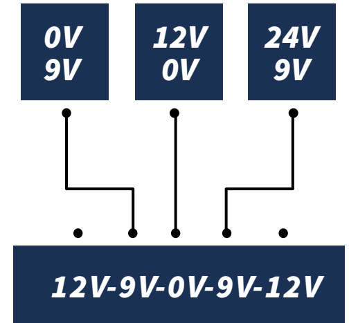
Transformer
